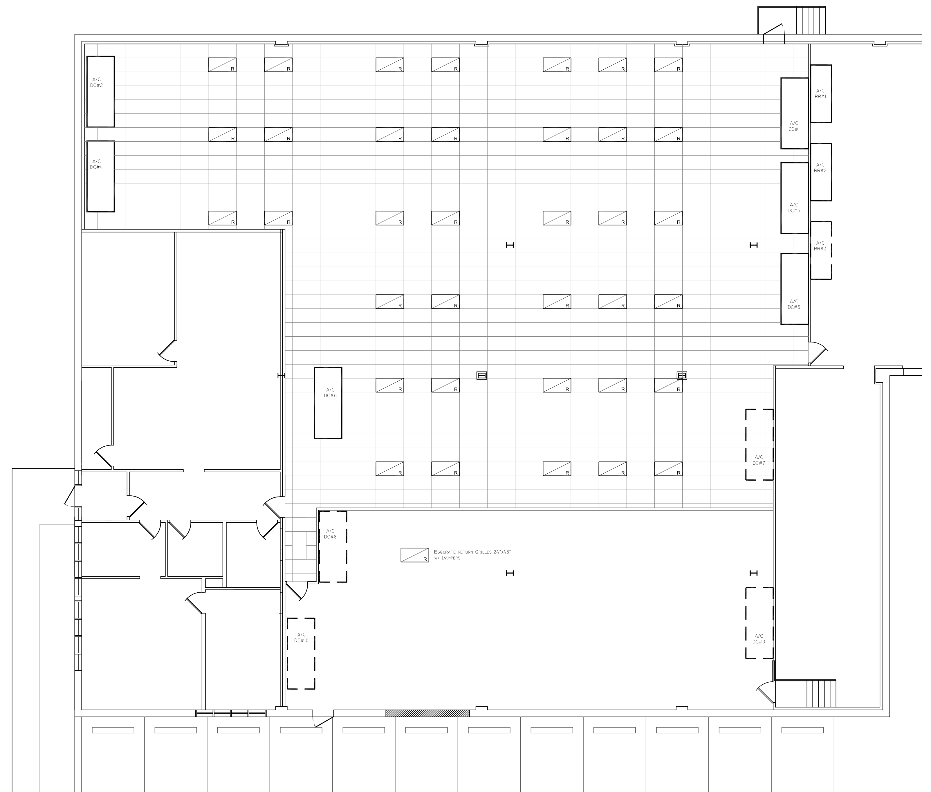
Return Grilles Layout Plan at Suspended Ceiling
