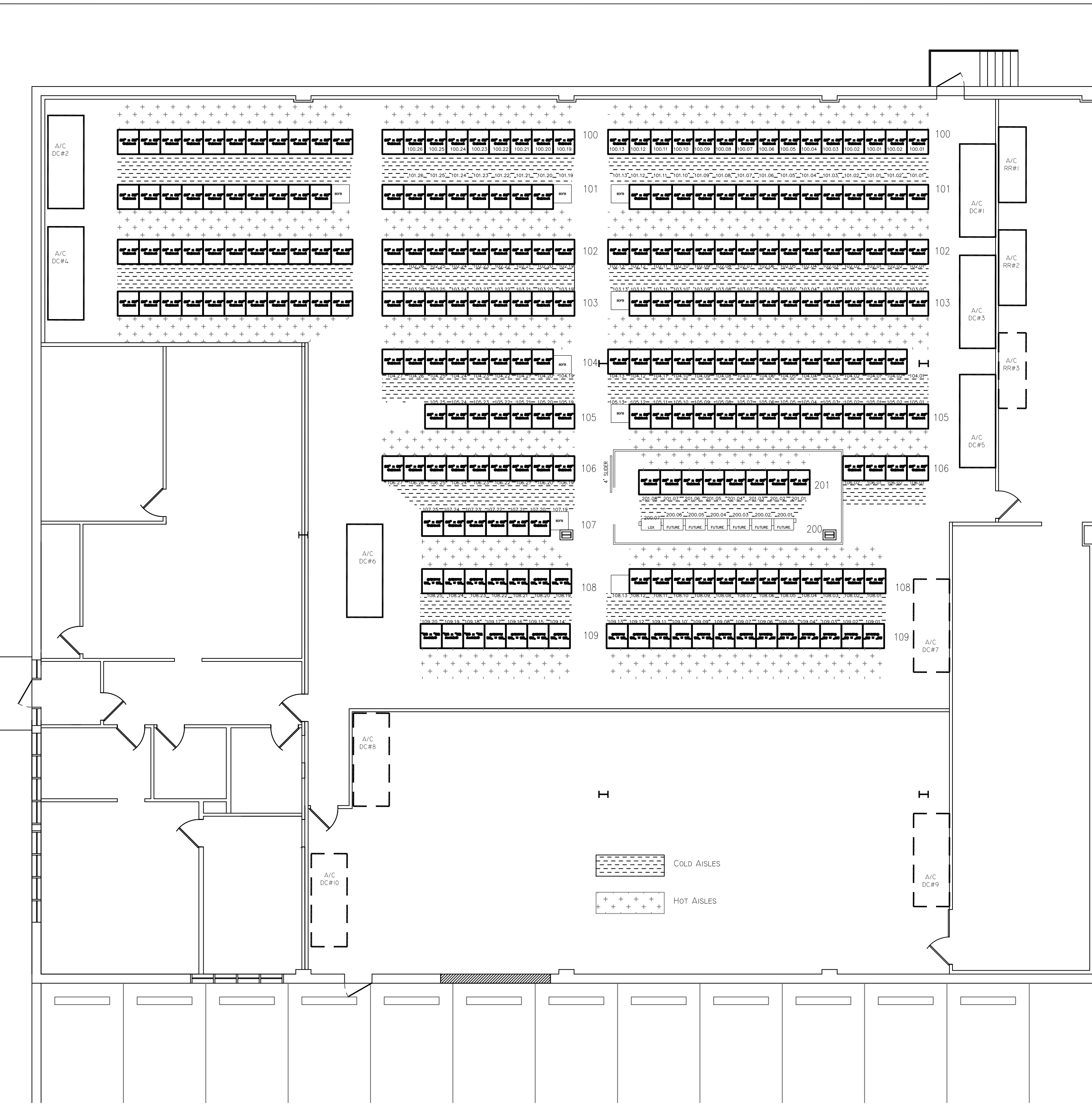
Hot/Cold Aisle Layout In Data Center
