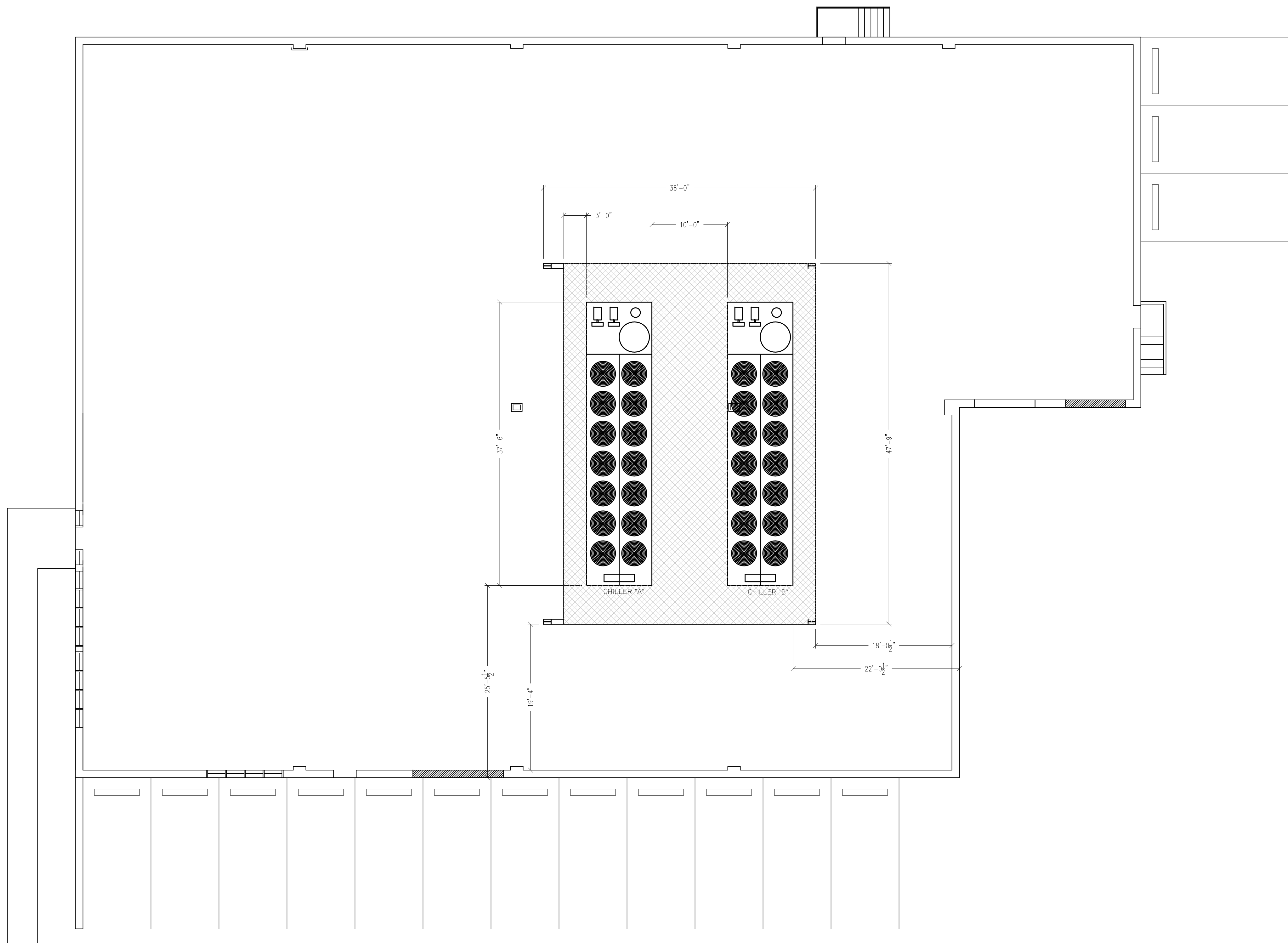
Layout For Chillers On Roof SCALE: 1/8"=1'-0"
