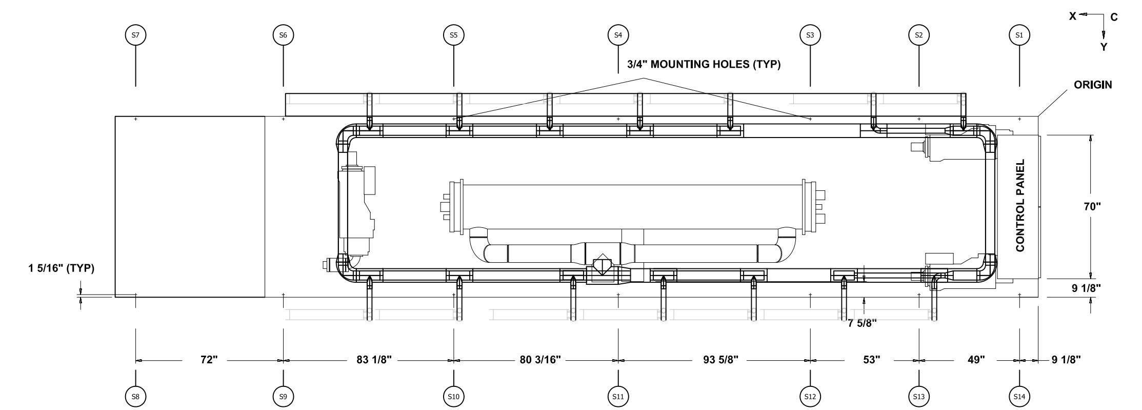
Equipment Details SCALE: 1/4"=1'-0"
